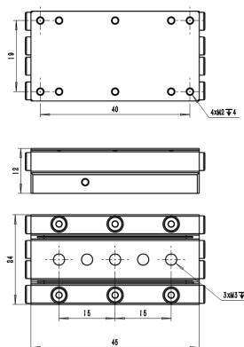
Applicable model: PMIN-C24X-20A / PMIN-C24X-30A Unit: mm
